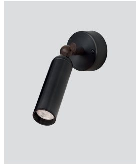
PATINA SPOT D. Pipe 40 mm D. Wall mounted 75 mm L. 240 mm Max 4 W GU10 35 mm 4200-18 Black oxide/oxide brass
